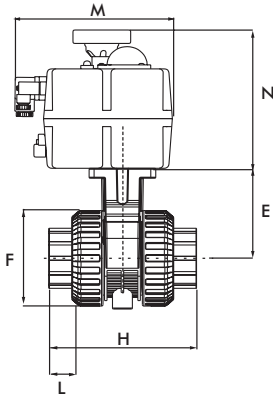
Actuator coupling dimensions (T4.2)
