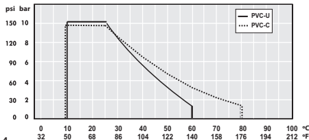
DN65 - DN100 (PVC-U, CPVC) (G 3.2)
